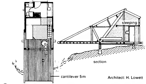
⑥ Timber weekend house for four people, 25 m² living area
